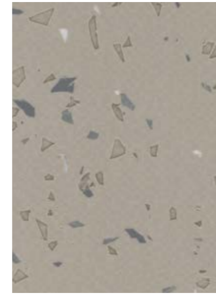
COSMIC - 4037 Gyptis
