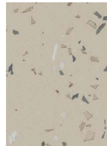
COSMIC - 4370 Palma
