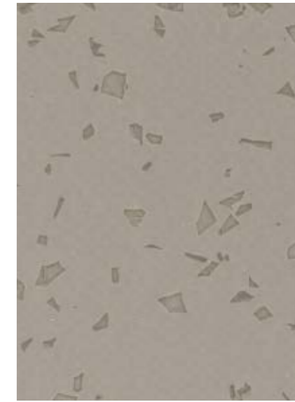
STELLAR - 4373 Fudo
